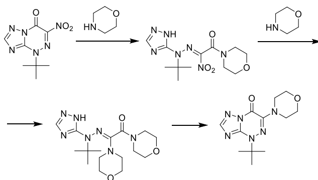
Scheme 20. ANRORC process of the nitro group substitution in N-alkyl substituted nitroazotriazines.
