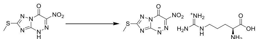
Scheme 7. Synthesis of L-arginine salt of TZV.
