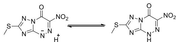
Scheme 5. Acidic NH-form of TZV.
